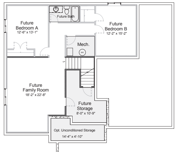
Basement Level
