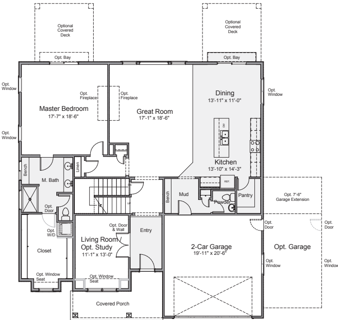
Main Level
