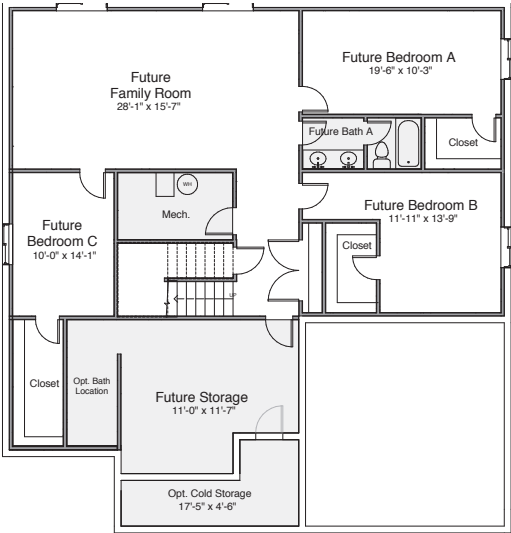
Basement Level
