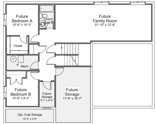
Basement Level
