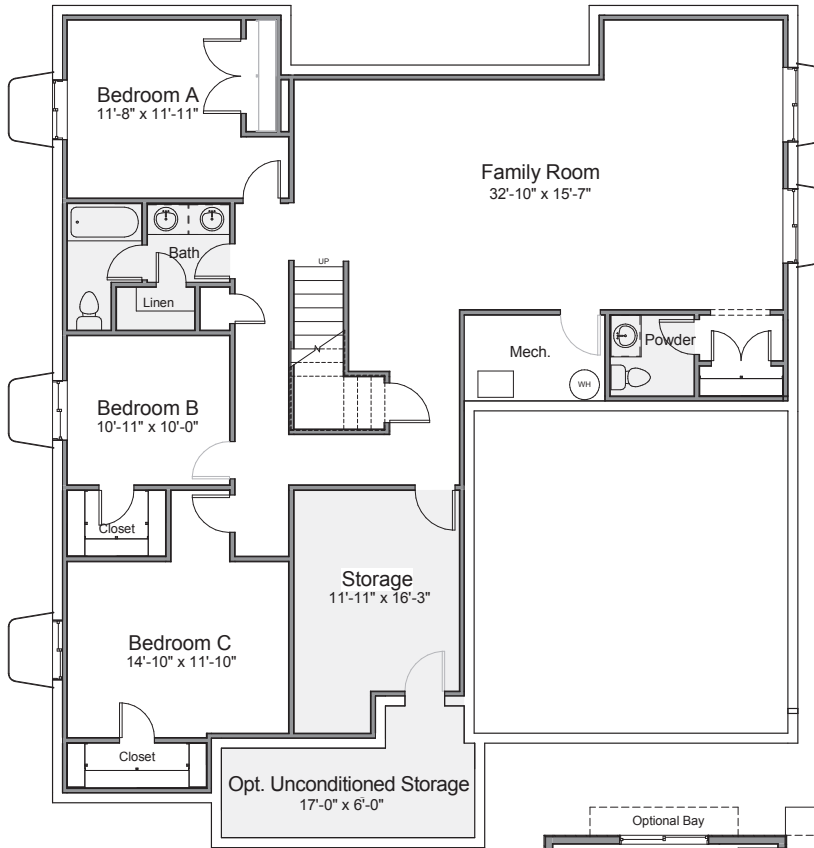
Basement Level
